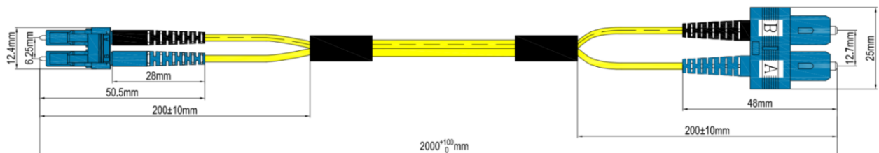
Dimensional drawing
