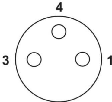
Pin assignment
